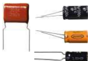
CAPACITOR 44.6055 Bipolar 47x100V KIT C/10 44.6054 Bipolar 100x100V KIT C/10 44.6065 Drive 2,2x250V KIT C/10
